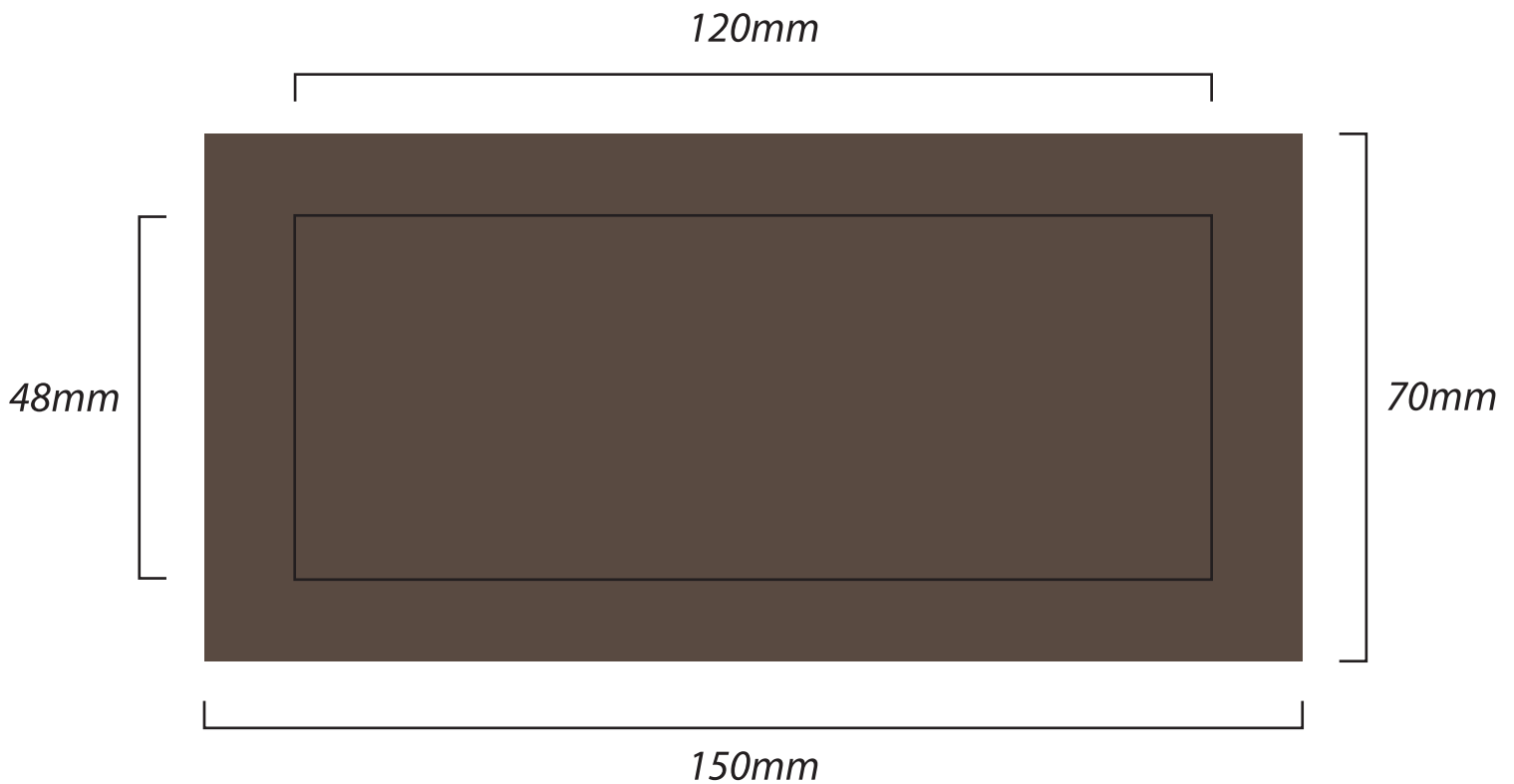
Top View
